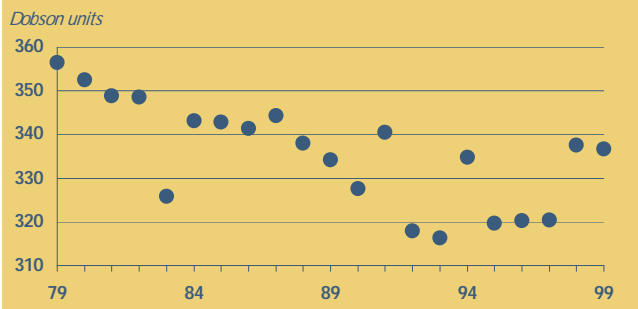
The Dobson ozone over Denmark
